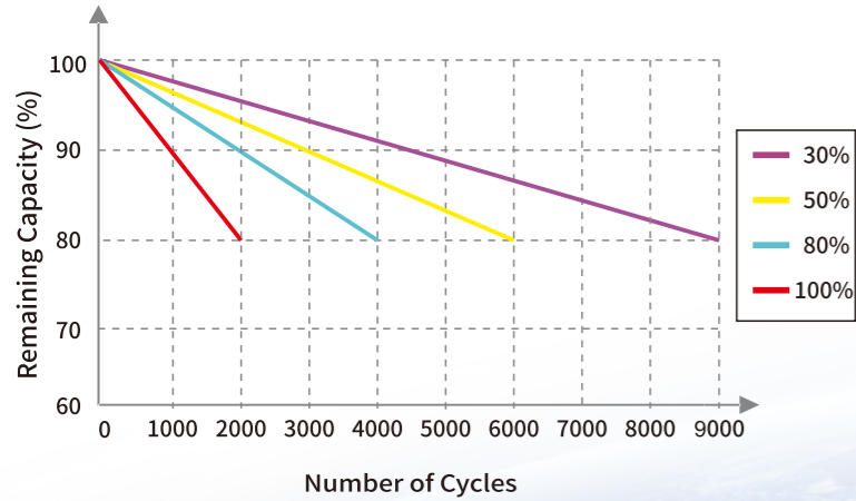
Different DOD Discharge Cycle Life Curve @1C
